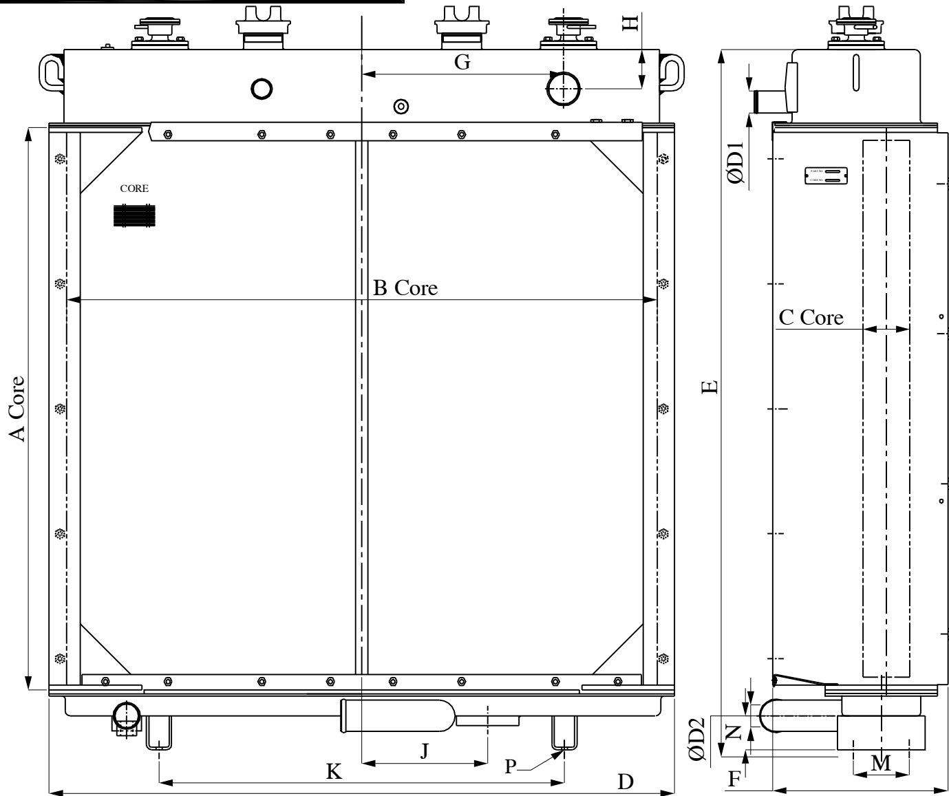
DIMENSIONAL DETAILS (MM)
